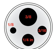
Multi-hole type 2 (CTC-320 A / 650 A)
