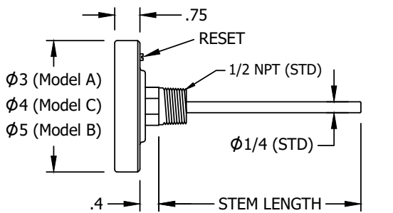
Standard Dimensions
