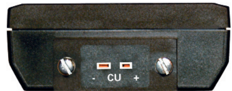
The TC-100 accepts both Mini-plug AND bare thermocouple wires
